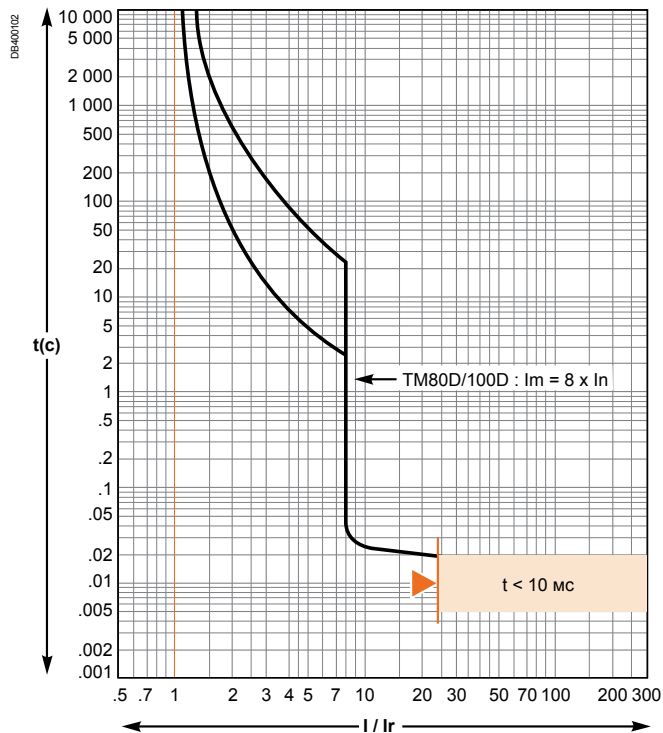
TM80D/100D
