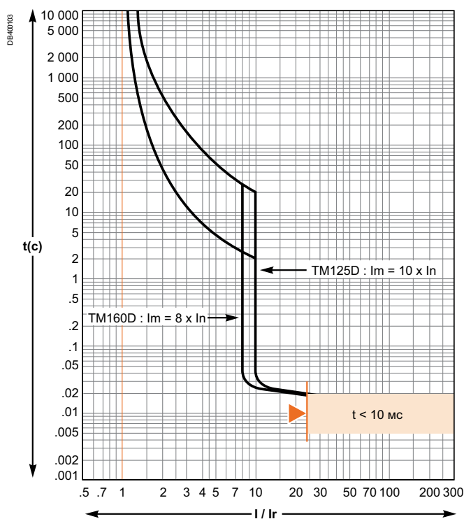
TM125D/160D
