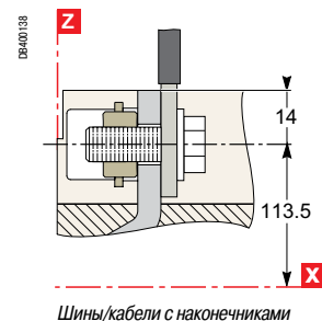
CVS400/630
