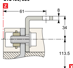
CVS400/630
